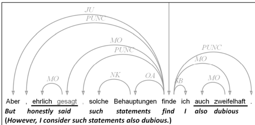
Figure 2. Dependency tree for Example 2
