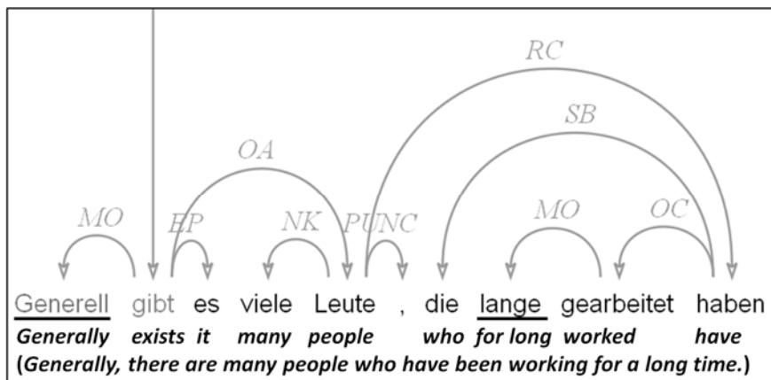
Figure 1. Dependency tree for Example 1
